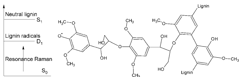
FIGURE 1 Simple model of lignin fragment with a reactive radical site and neutral sites. The electronic state energy diagram illustrates that the radical is selectively probed by resonance excitation due to its low-lying electronic excited D_1 state.
